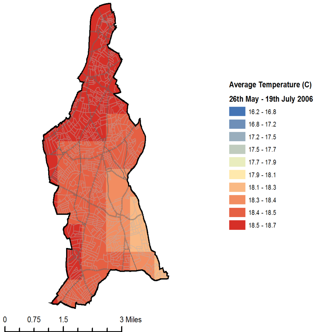
Figure 6: Average temperatures in Lambeth
